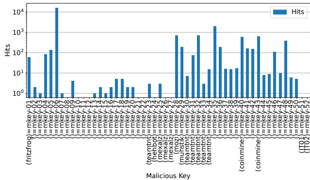
Figure 8: Malicious key count, port 22
