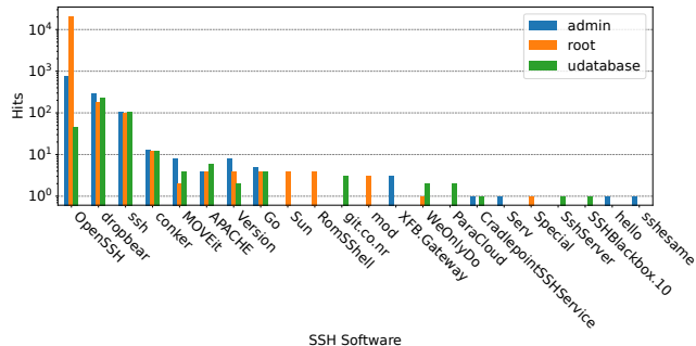
Figure 4: SSH server implementation vs. username, port 22
