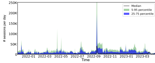
(a) NO_CRED
