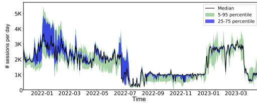
(c) NO_CMD
