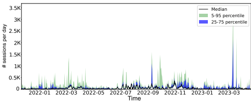
(e) CMD+URI
