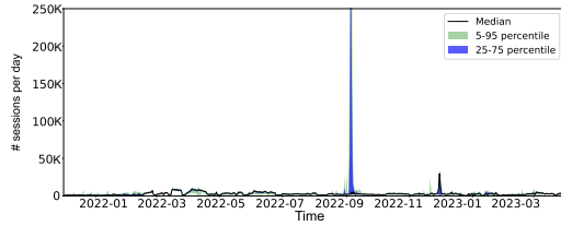
(b) FAIL_LOG
