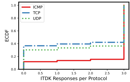
Figure 6: Responsiveness per protocol for the ITDK dataset.
