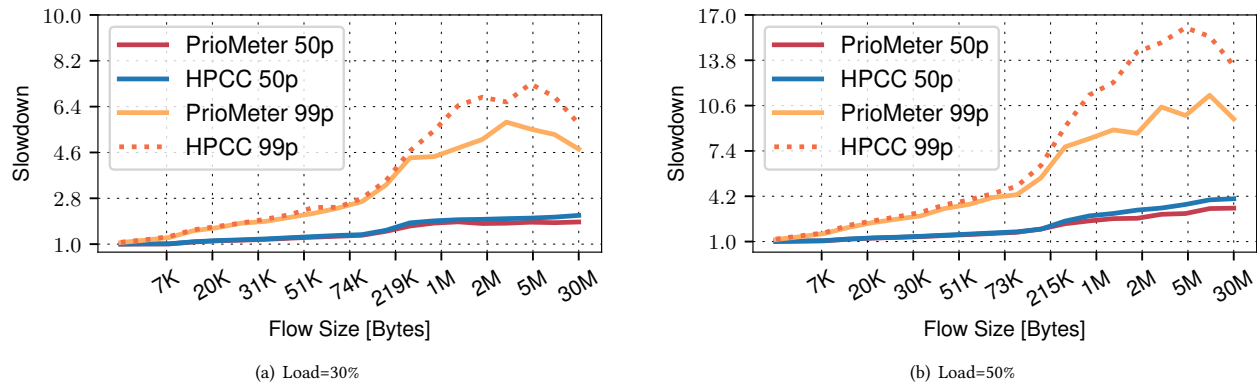
Figure 6: The FCT slowdown for PRIOMETER and HPCC on webSearch workload for 50- and 99-FCT percentiles. when the link loads are 30% and 50%.
